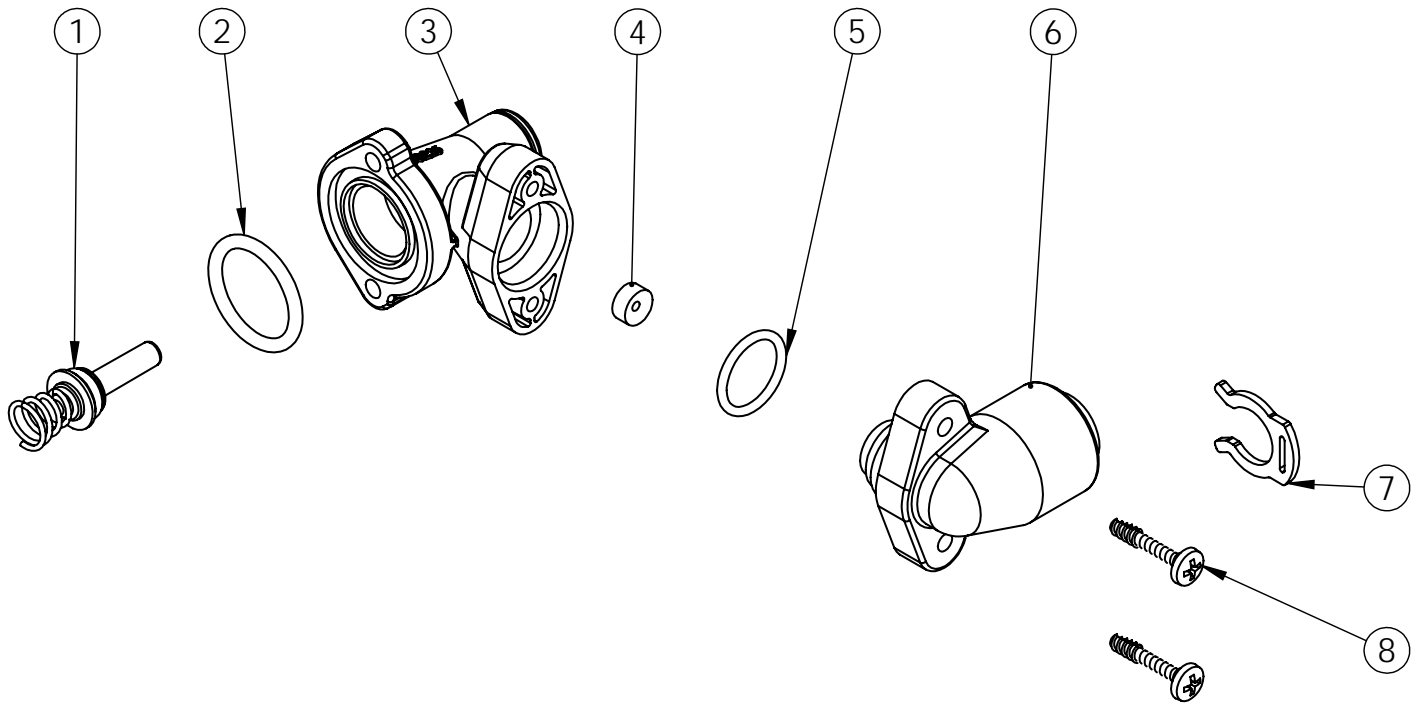
Figure 11: Brine Valve Housing Assembly
