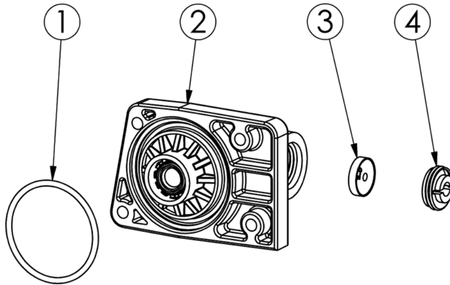
Figure 12: Drain End Cap Assembly
