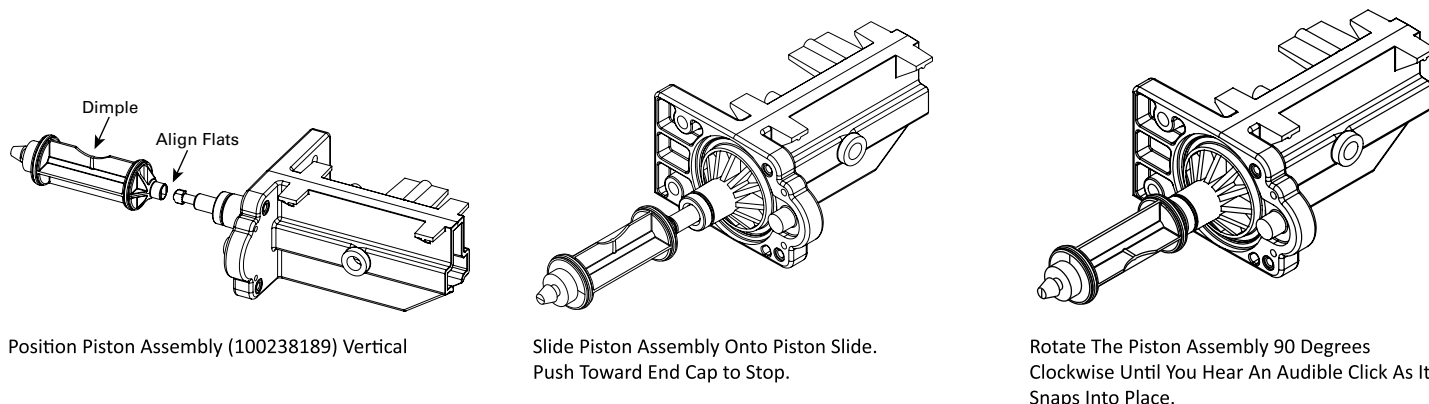
Figure 10: Piston Slide Assembly
